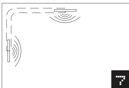
90° TURN TRACK ADJACENT WALLS
