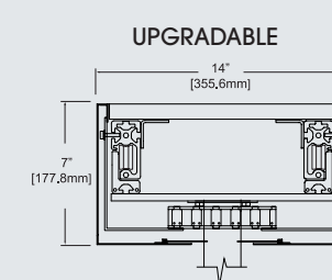
RECESSED MOUNT MANUAL SUPER TRAK
