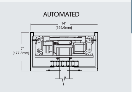
RECESSED MOUNT AUTOMATED SUPER TRAK
